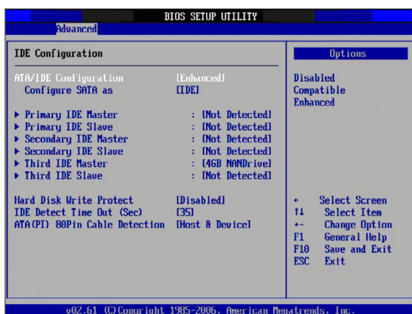
Figure 3.5 IDE Configuration
