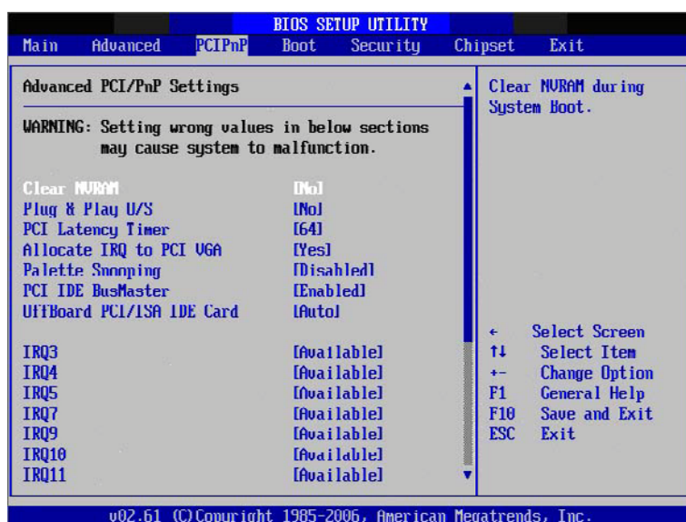
Figure 3.20 PCI/PNP Setup
