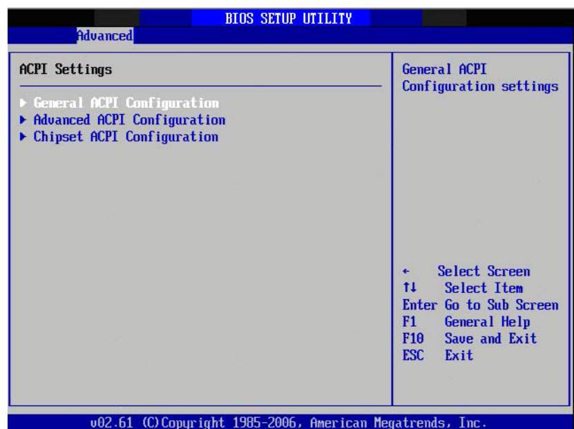
Figure 3.9 ACPI Settings
