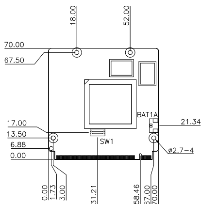
Component Side
