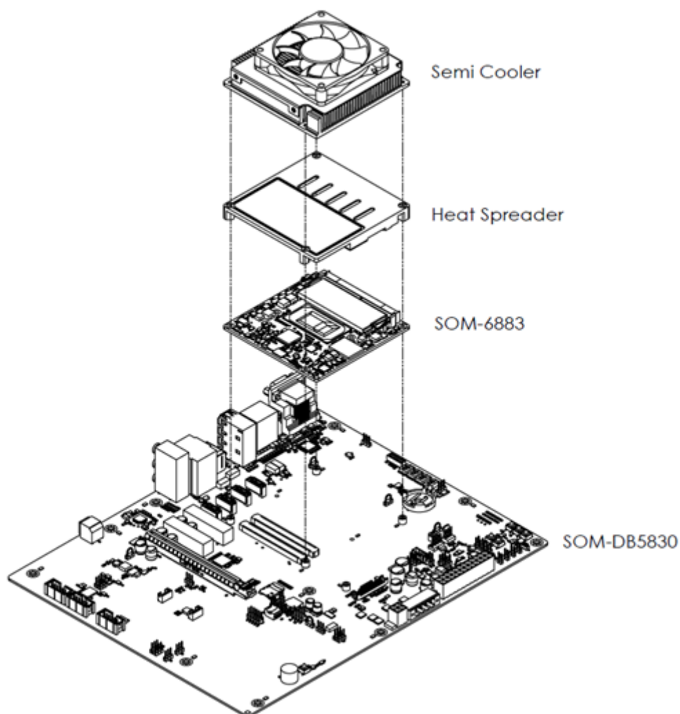
Figure 2.6 Assembly Diagram
