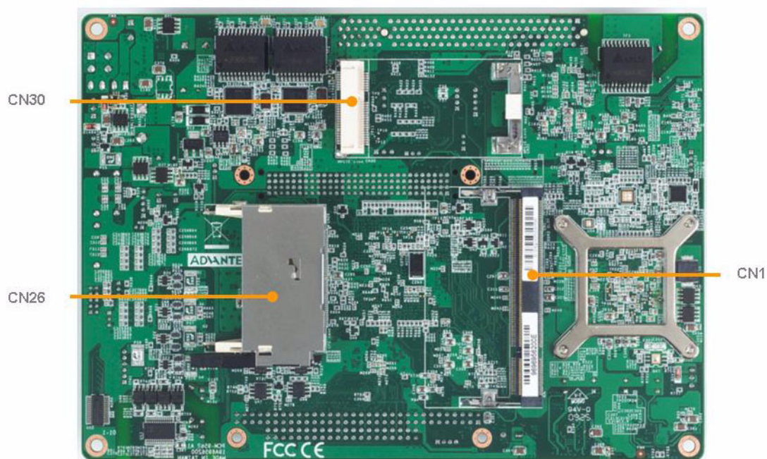
Figure 2.1 Jumper and Connector Layout (Component Side)
