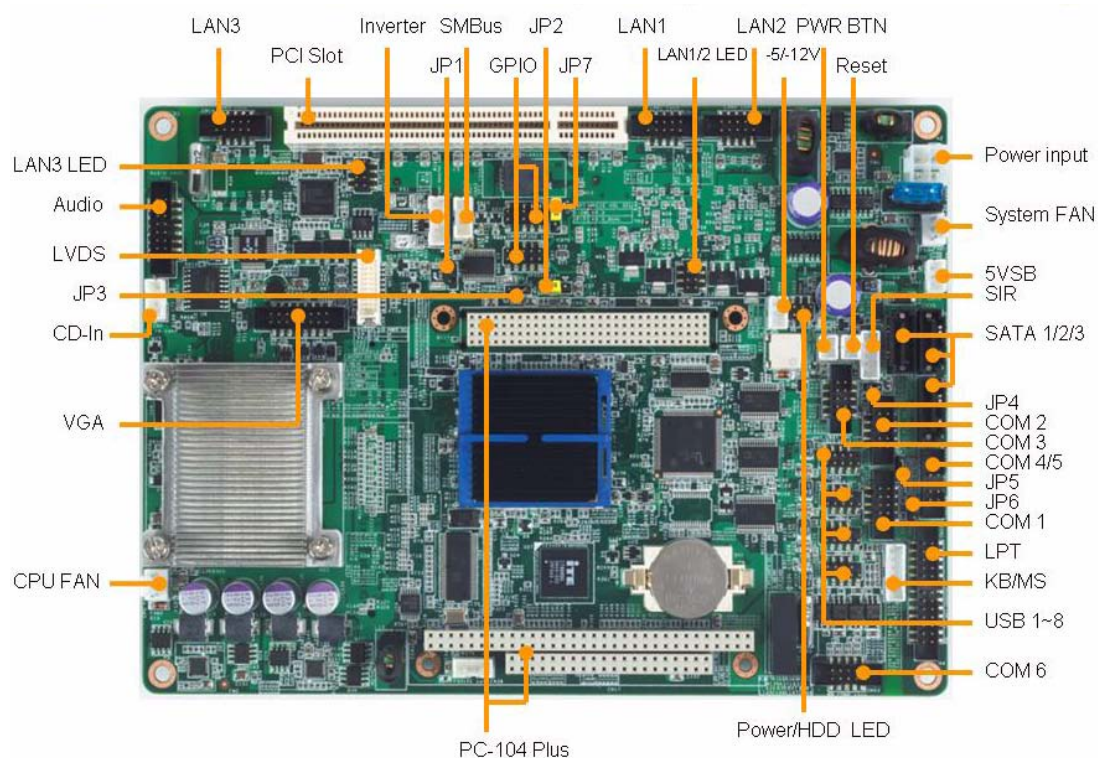
Figure 2.1 Jumper and Connector Layout (Component Side)
