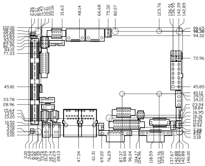
PCM-9362 Mechanical Drawing (Component Side)
