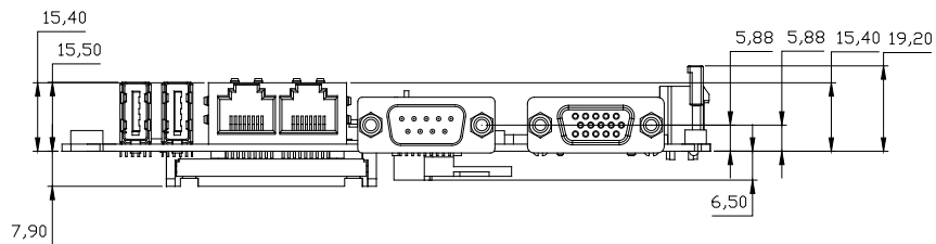
PCM-9362 Mechanical Drawing (Side View)
