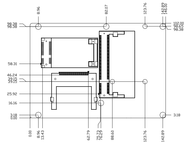
PCM-9362 Mechanical Drawing (Solder Side)
