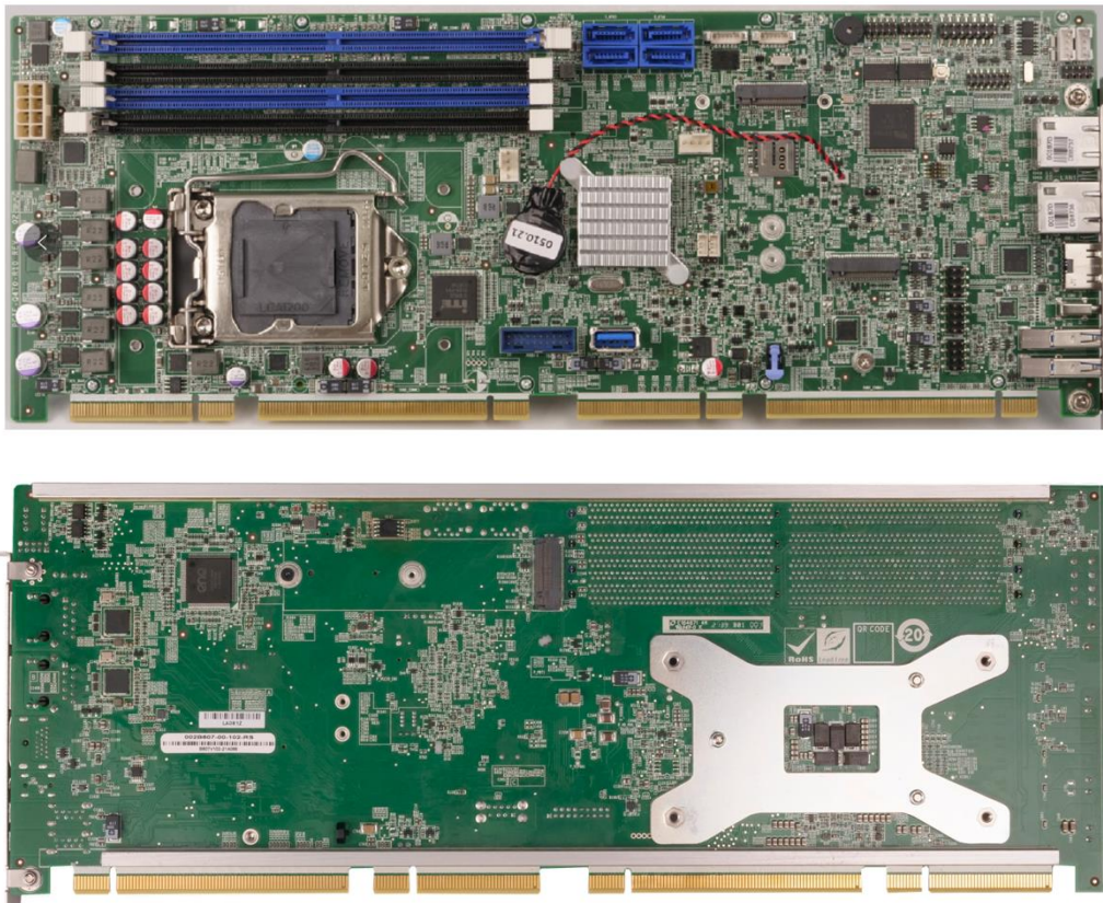
Figure 1-1: PCIE-Q470
