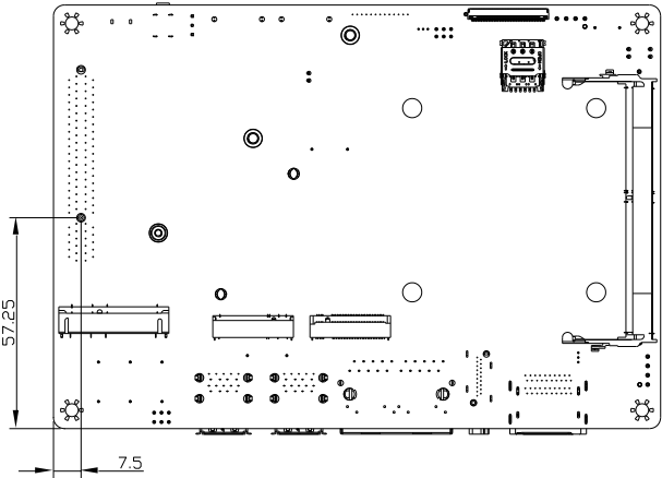
Solder Side
