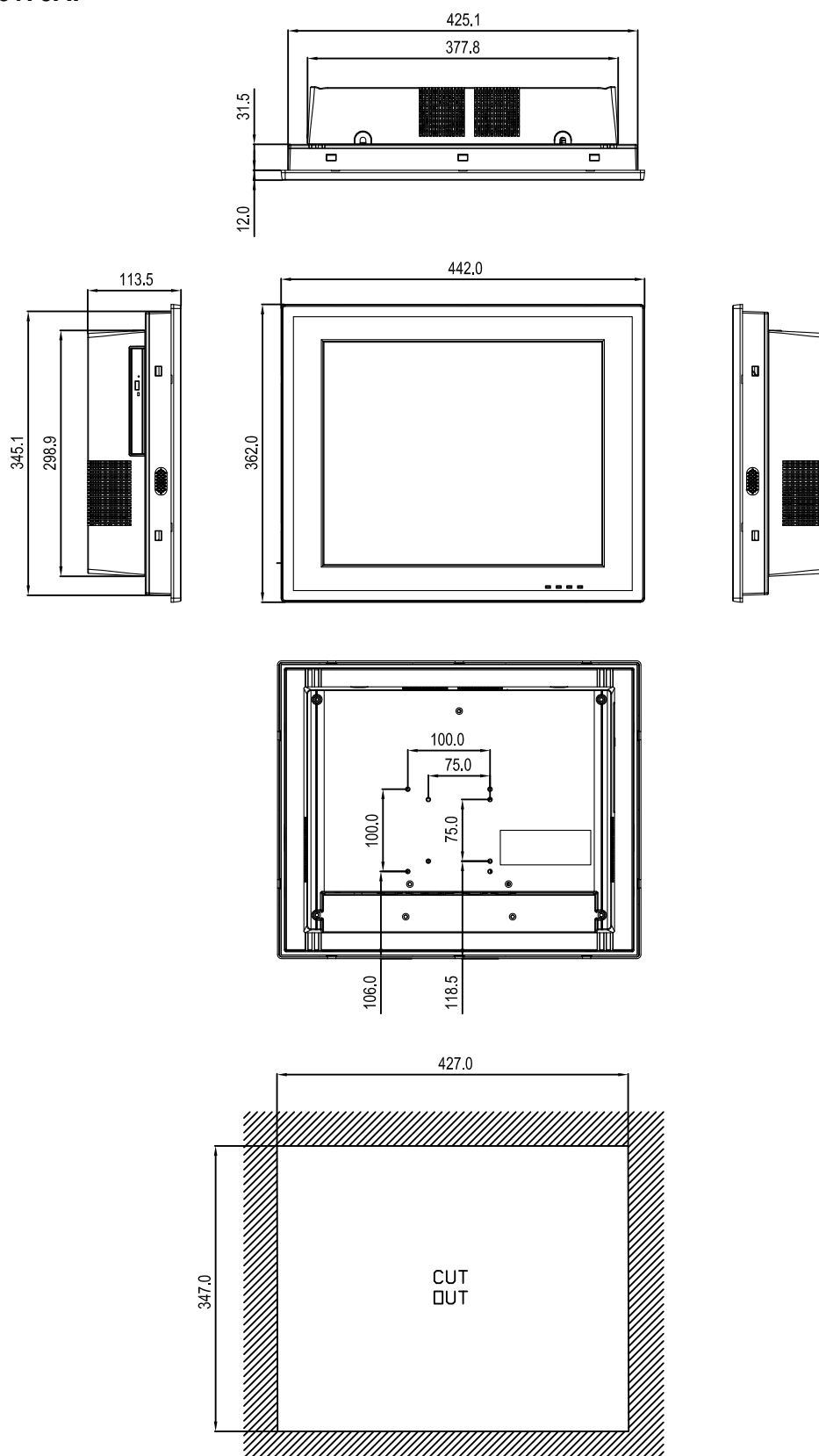
Figure 1.2 PPC-6170A dimensions
