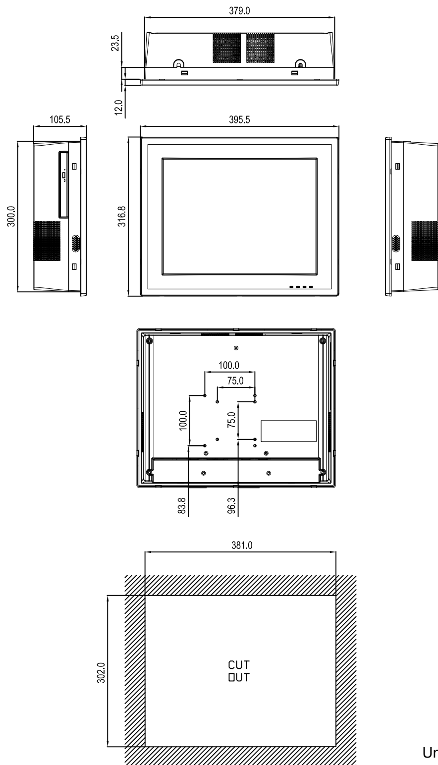
Figure 1.1 PPC-6150A dimensions
