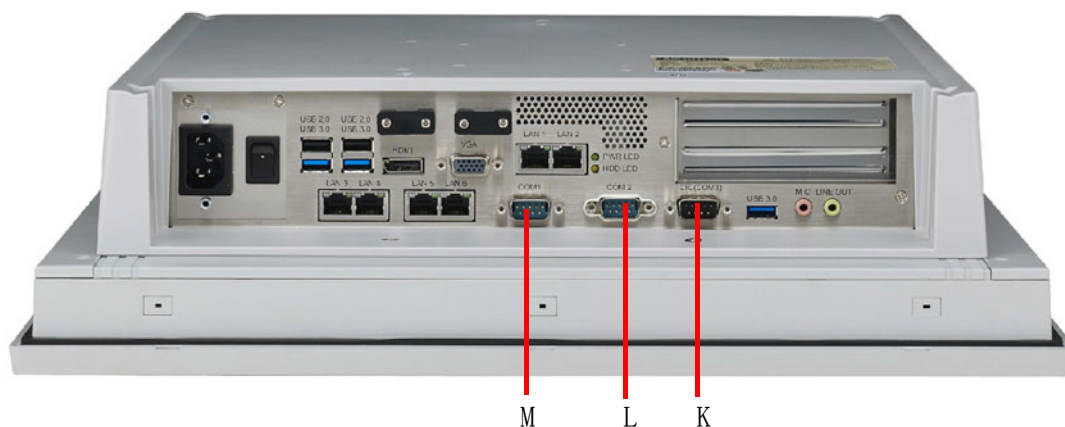
Figure 3.4 COM ports
