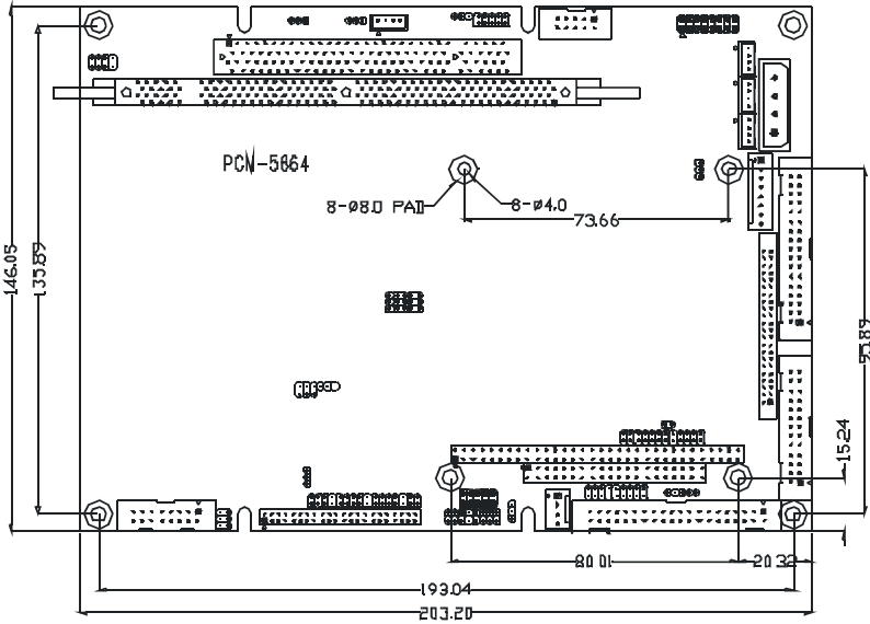
Figure 1-1: PCM-5864/L dimensions
