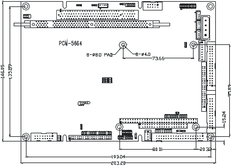
Figure 1-1: PCM-5864/L dimensions
