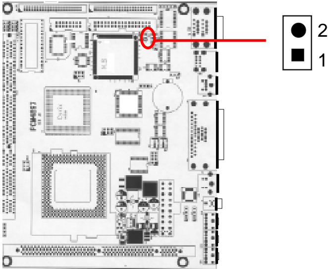
LCD Backlight power connector (J1)
