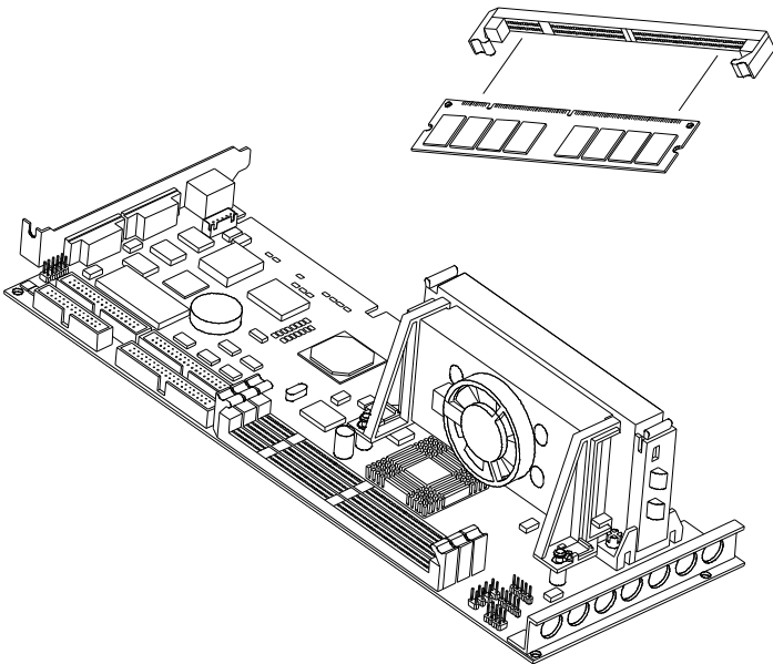
Figure 1-3: DIMM installation
